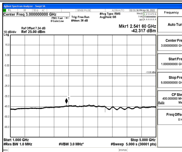
Band5-10MHz-QPSK-20600-1-0-High-1000-5000--42.32-PASS
