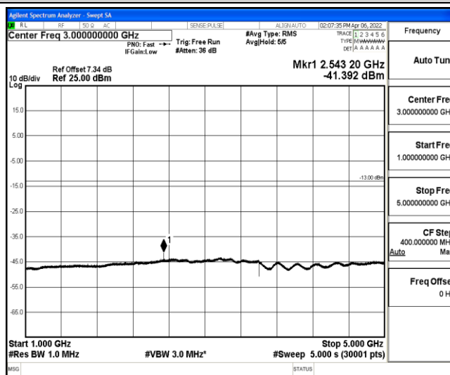
Band5-5MHz-16QAM-20625-1-0-High-1000-5000--41.39-PASS
