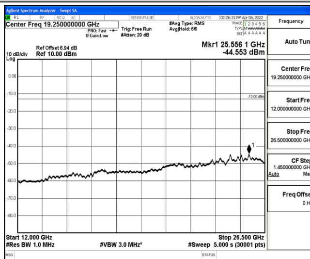
Band5-10MHz-16QAM-20450-1-0-Low-12000-26500--44.55-PASS
