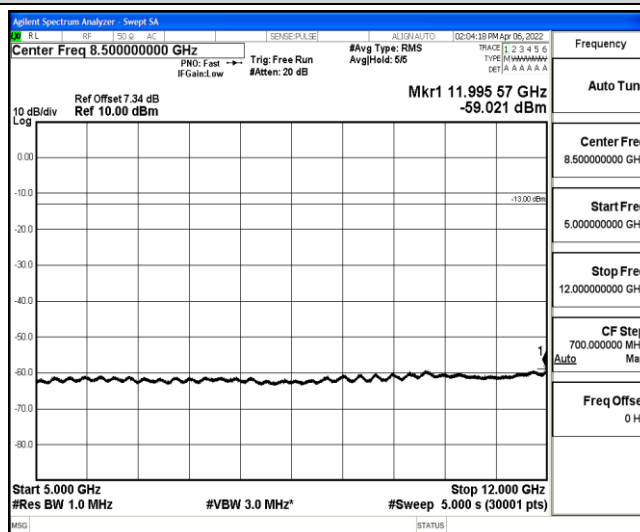
Band5-5MHz-16QAM-20525-1-0-Low-5000-12000--59.02-PASS
