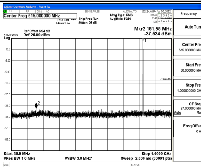
Band5-10MHz-16QAM-20450-1-0-Low-30-1000--37.53-PASS
