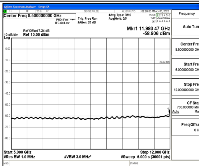
Band5-10MHz-QPSK-20525-1-0-Low-5000-12000--58.91-PASS
