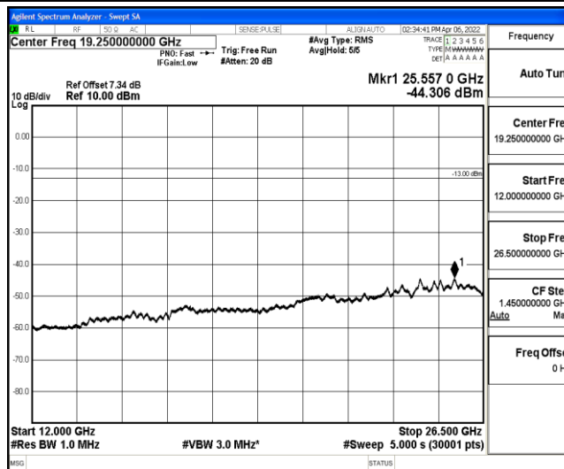
Band5-10MHz-16QAM-20600-1-0-High-12000-26500--44.31-PASS
