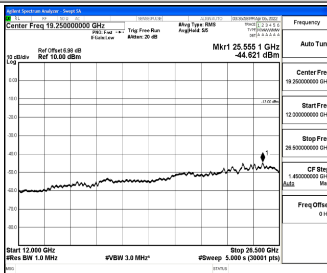
Band12-3MHz-16QAM-23025-1-0-Low-12000-26500--44.62-PASS
