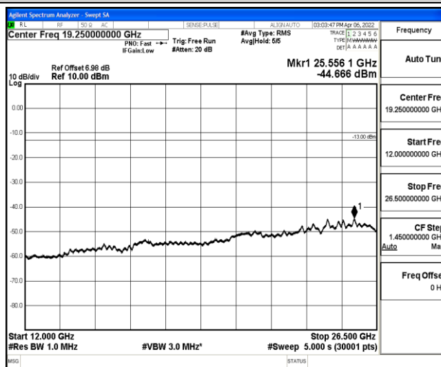
Band12-1.4MHz-16QAM-23017-1-0-Low-12000-26500--44.67-PASS
