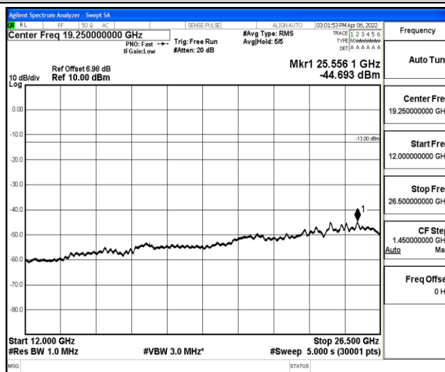
Band12-1.4MHz-QPSK-23017-1-0-Low-12000-26500--44.69-PASS
