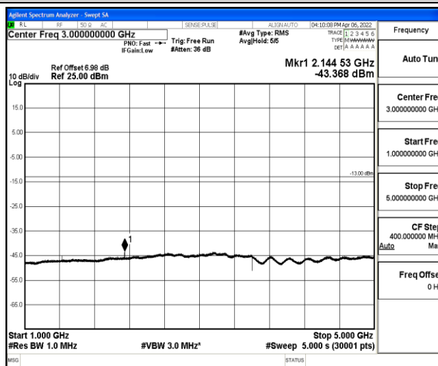
Band12-5MHz-QPSK-23155-1-0-High-1000-5000--43.37-PASS
