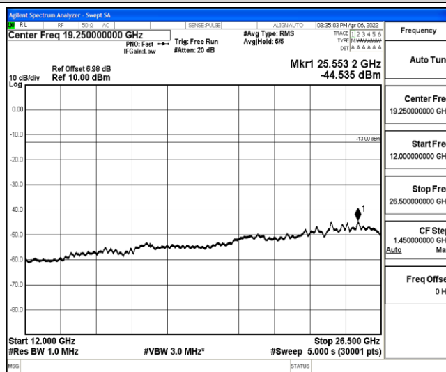
Band12-3MHz-QPSK-23025-1-0-Low-12000-26500--44.54-PASS
