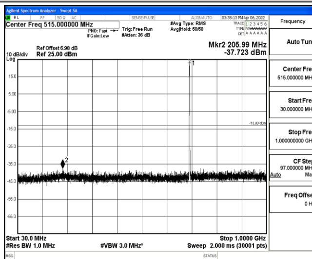
Band12-3MHz-16QAM-23025-1-0-Low-30-1000--37.72-PASS
