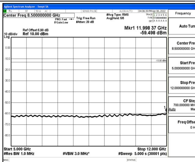
Band12-5MHz-QPSK-23095-1-0-Low-5000-12000--59.5-PASS
