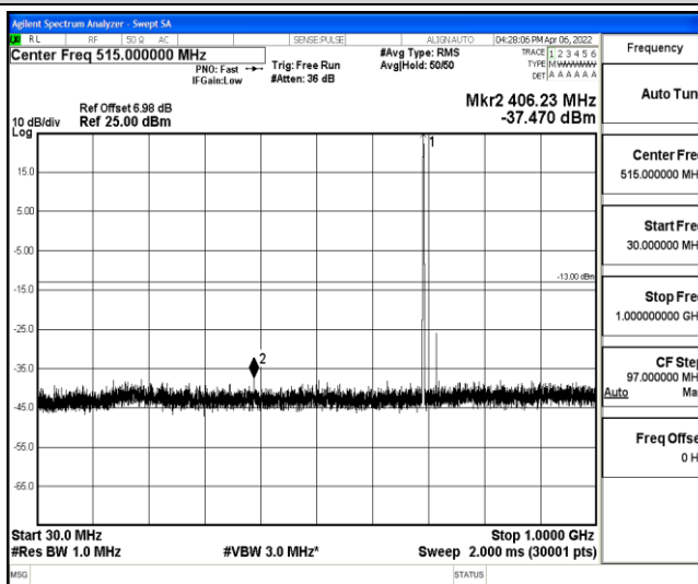
Band12-10MHz-16QAM-23060-1-0-Low-30-1000--37.47-PASS
