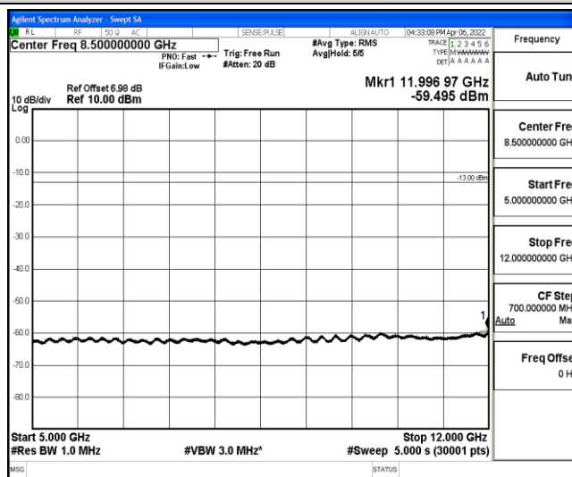
Band12-10MHz-16QAM-23095-1-0-Low-5000-12000--59.5-PASS
