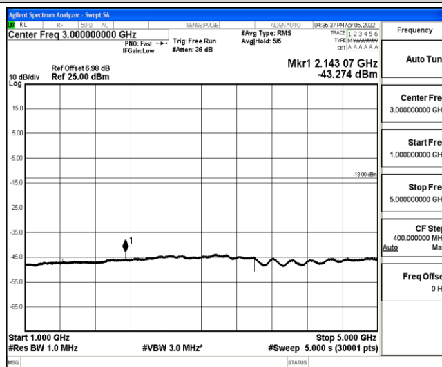
Band12-10MHz-16QAM-23130-1-0-High-1000-5000--43.27-PASS
