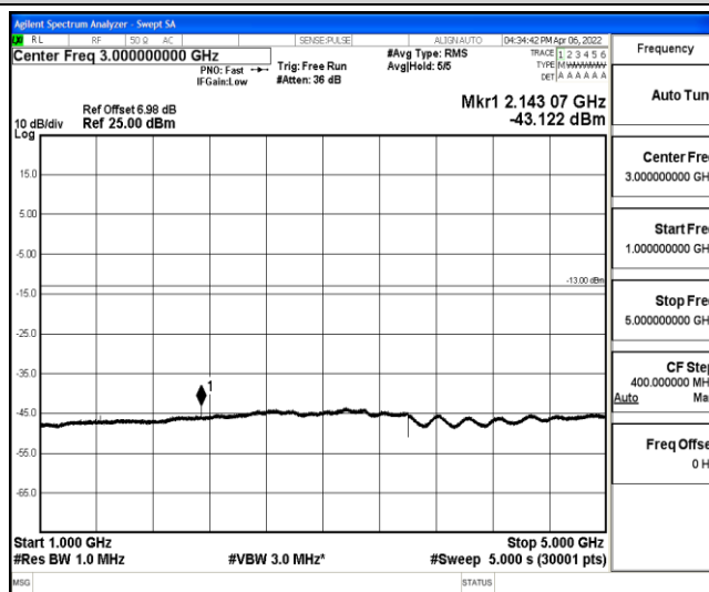
Band12-10MHz-QPSK-23130-1-0-High-1000-5000--43.12-PASS
