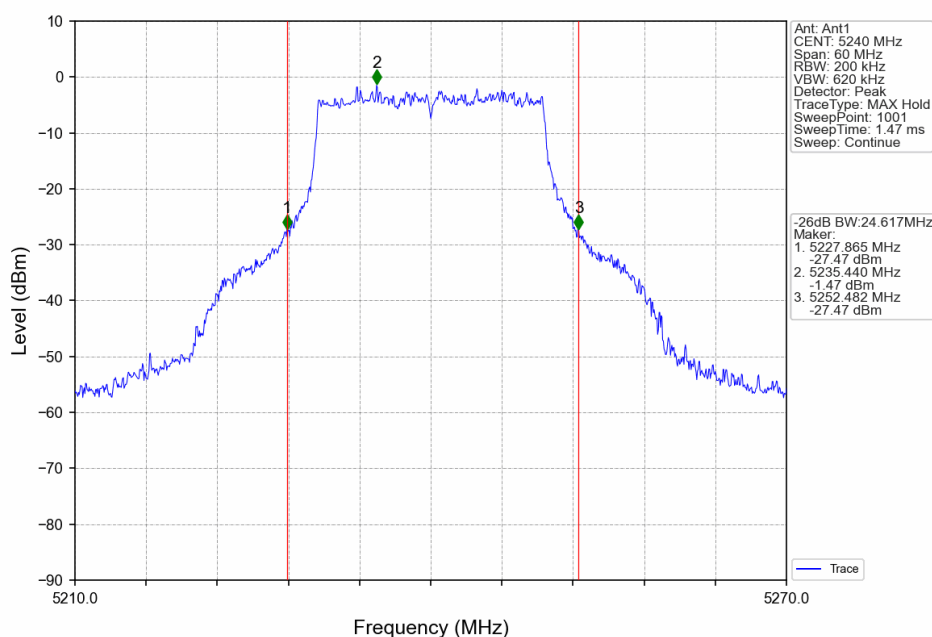
802.11ax(HEW20)_HCH_5240MHz_RU242_Left_Ant1_NTNV
