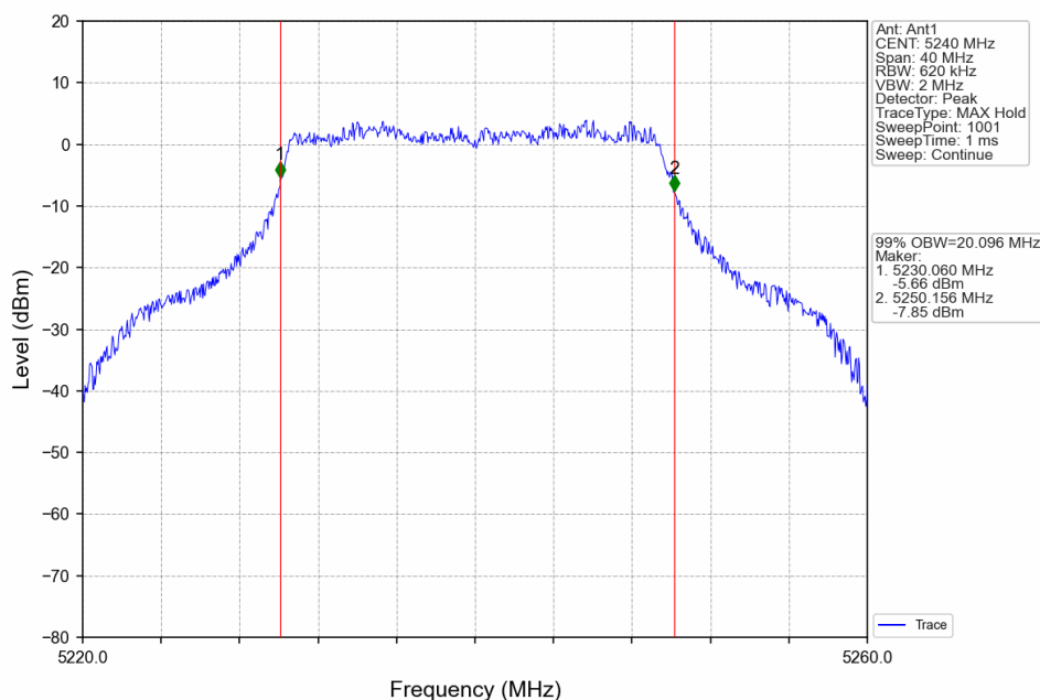
802.11ax(HEW20)_HCH_5240MHz_RU242_Left_Ant1_NTNV
