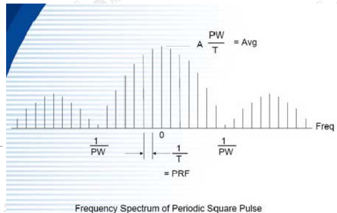
Frequency Spectrum of Periodic Square Pulse
