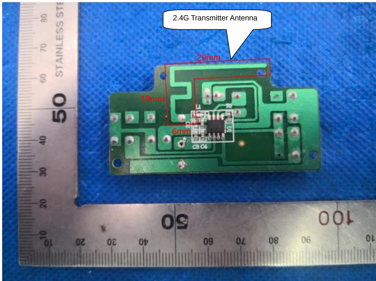
INTERNAL VIEW OF EUT (FIGURE 2)
