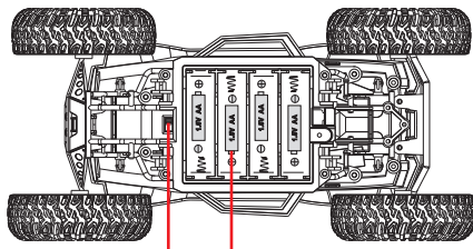
ON/OFF 4X1.5V AA Batteries (SWITCH) (Not included)
