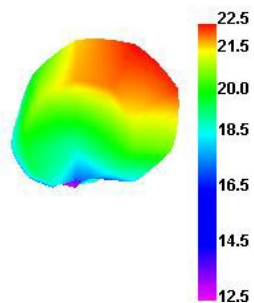
Wifi 1 TRP
