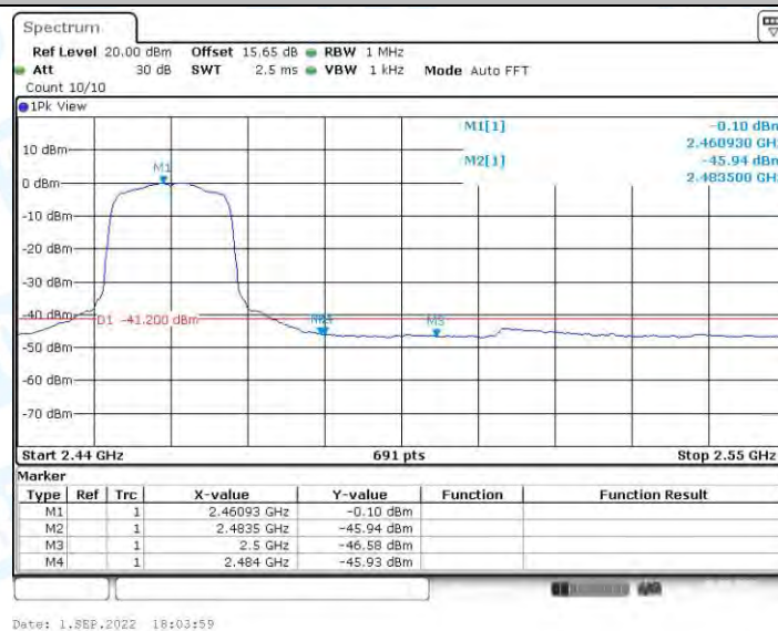
11G-CDD_Ant2_High_2462_Peak
