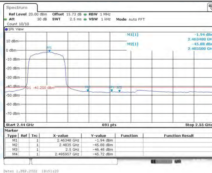
11N20MIMO_Ant1_High_2462_Peak
