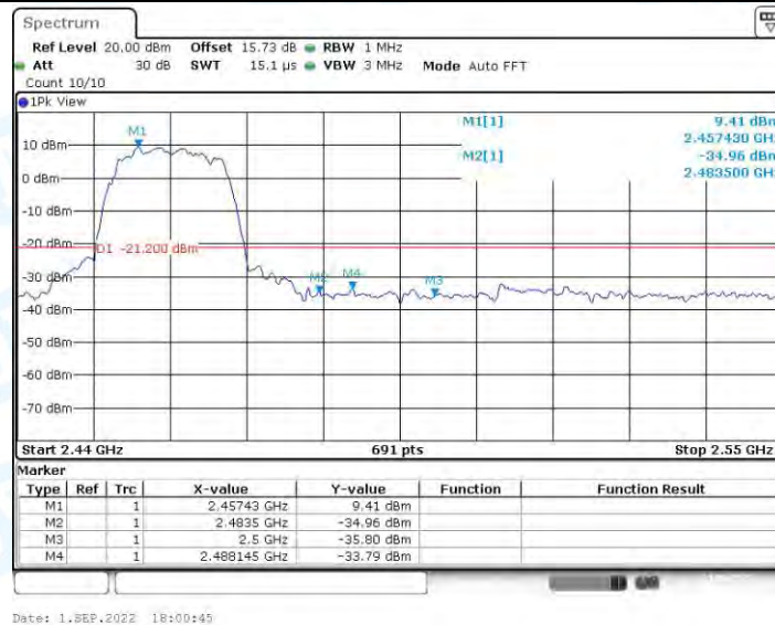
11G-CDD_Ant2_High_2462_AV
