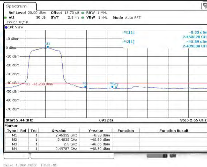
11G-CDD_Ant1_High_2462_Peak
