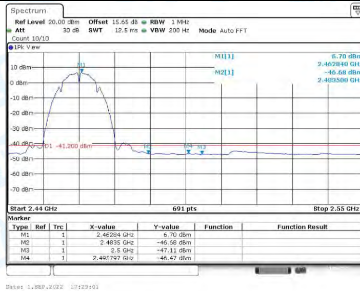
11B-CDD_Ant2_High_2462_Peak
