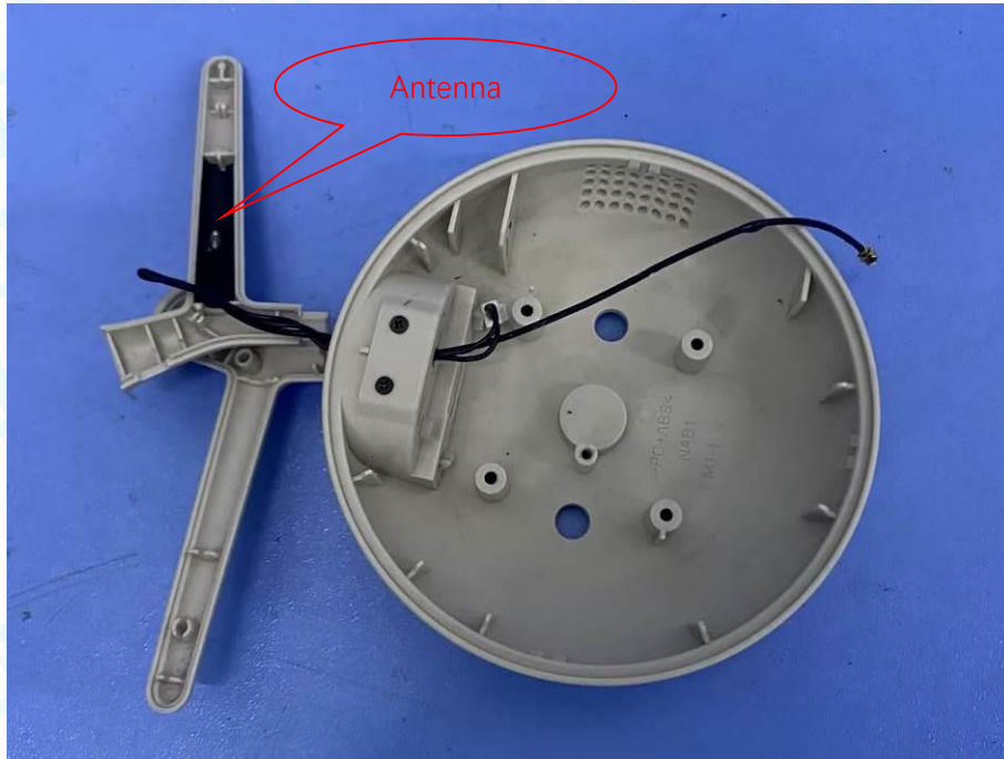
Photo 20 Internal of EUT
