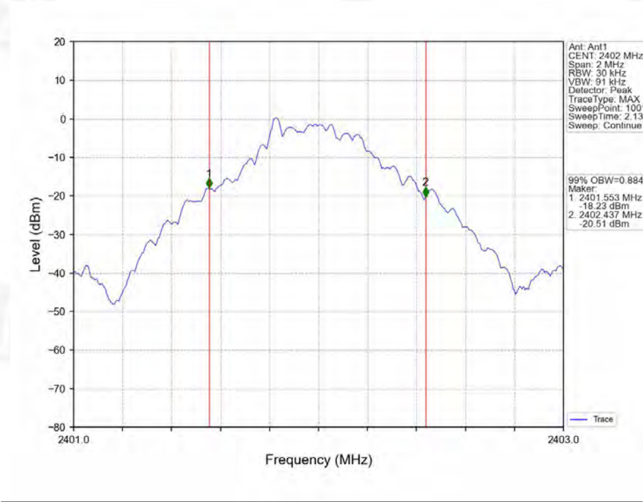
Test plots GFSK Low Channel
