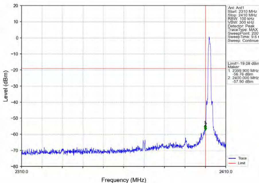
\pi/4 -DQPSK No-hopping Band edge-left side
