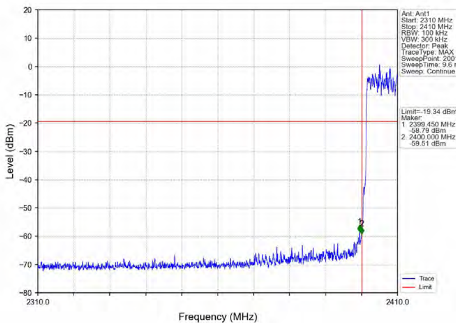
\pi/4 -DQPSK Hopping Band edge-left side
