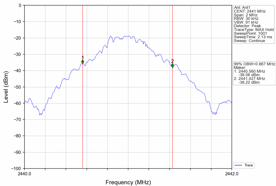
GFSK_DH5_MCH_2441MHz_Ant1_NTNV
