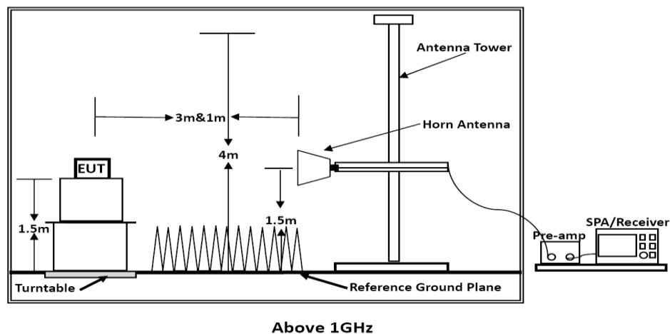
Radiated Emission Test Set-Up, Frequency above 1000MHz
