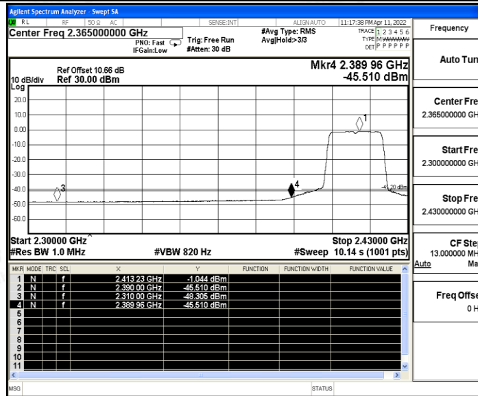
11N20SISO_Ant_Low_2412_Peak
