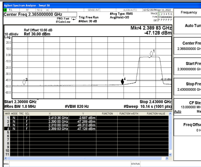
11G_Ant_Low_2412_Peak
