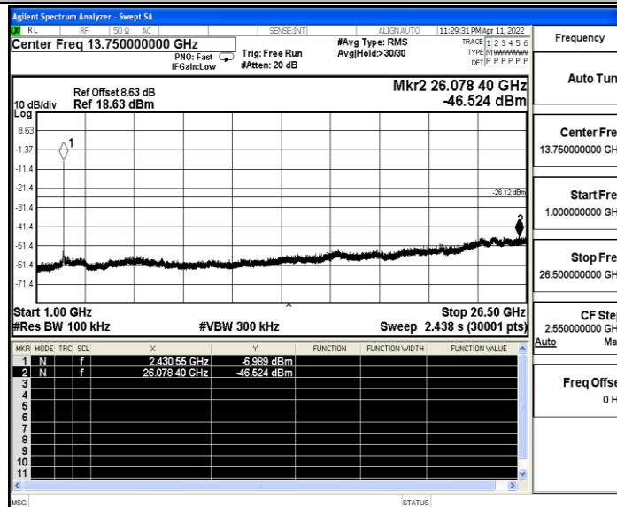
11N20SISO_Ant_2462_0~Reference
