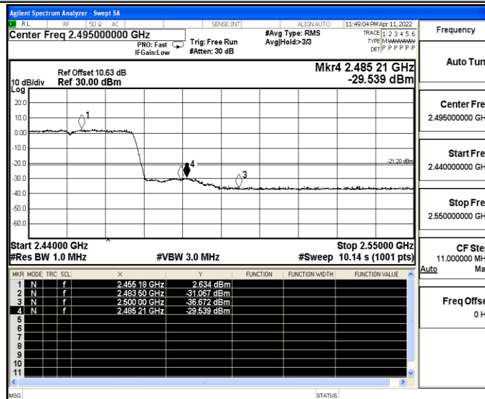
11N40SISO_Ant_High_2452_Peak
