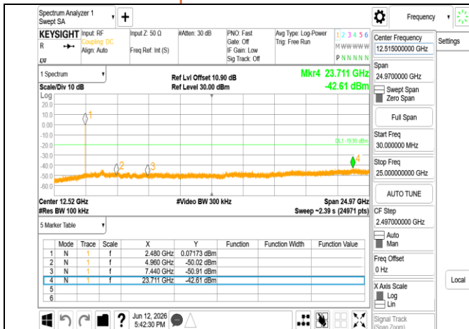
Spurious Emission_BLE_1M_HighCH39-2480
