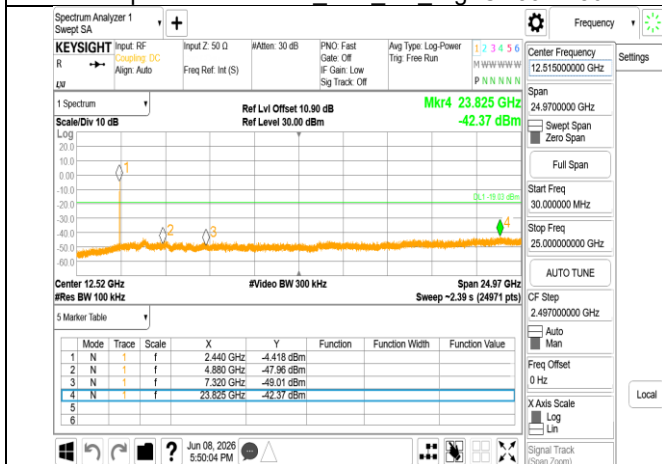
Spurious Emission_BLE_2M_MidCH19-2440
