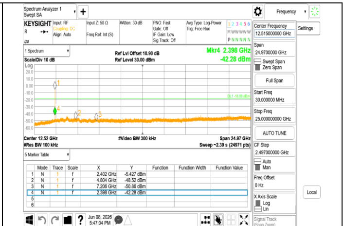
Spurious Emission_BLE_2M_LowCH00-2402
