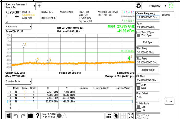
Spurious Emission_BLE_2M_HighCH38-2478
