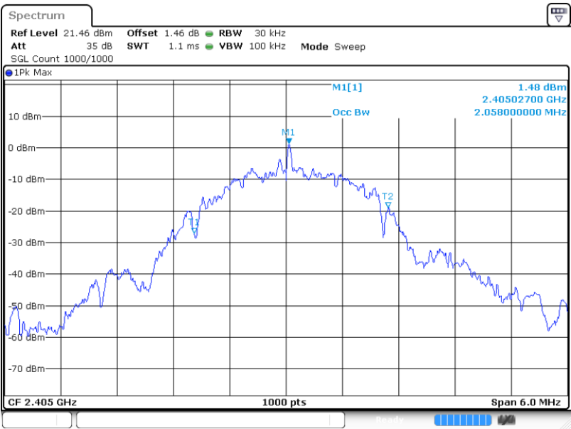
Low Channel (2405 MHz), 99% OBW
