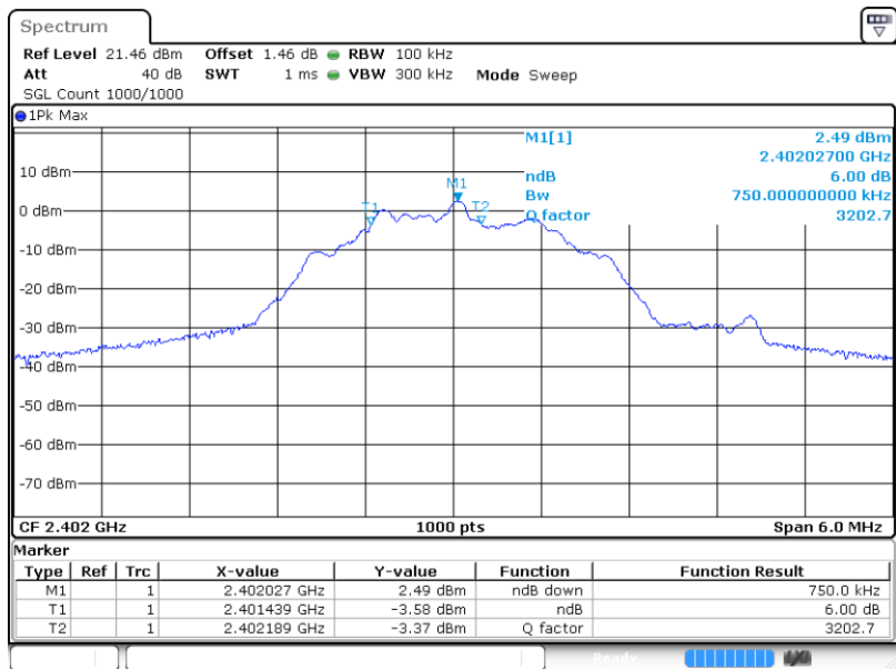
Low Channel (2402 MHz), -6 dB OBW
