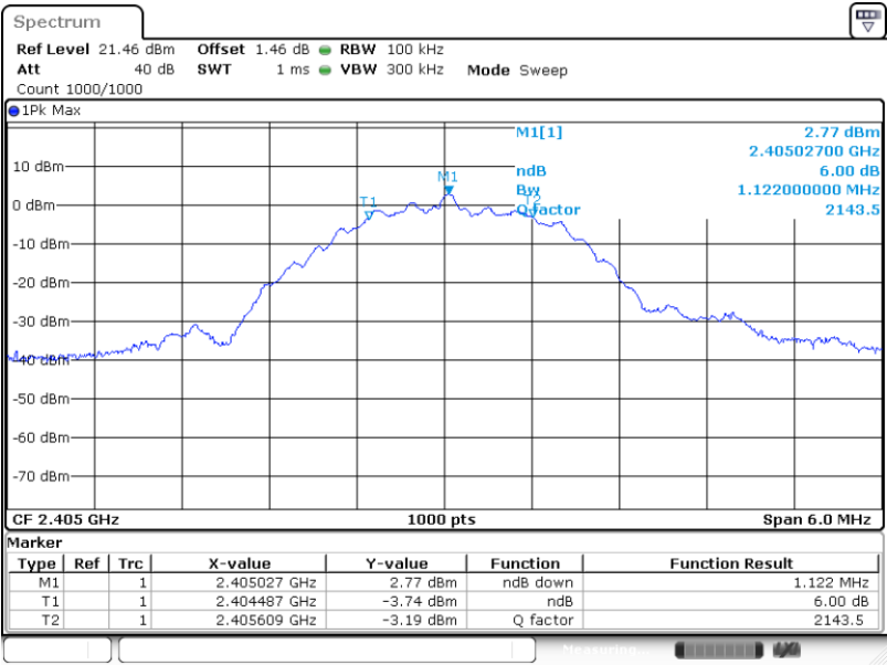
Low Channel (2405 MHz), -6 dB OBW
