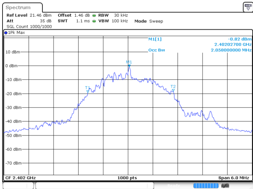
Low Channel (2402 MHz), 99% OBW
