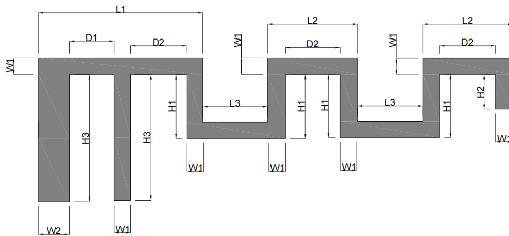
Antenna Dimensions
