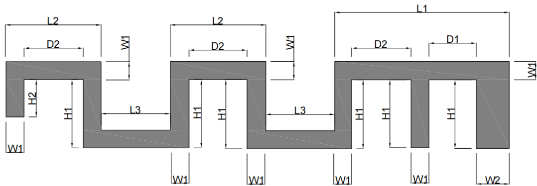
Antenna Dimensions
