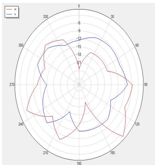
2490P90 Polar
