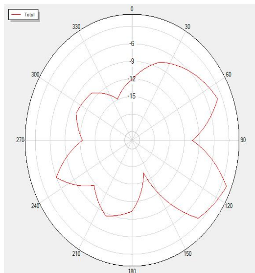
2430P0 Total
