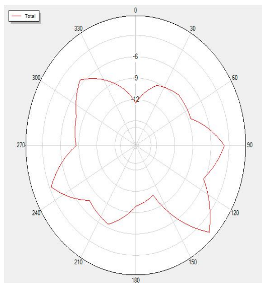
2500P90 Total
