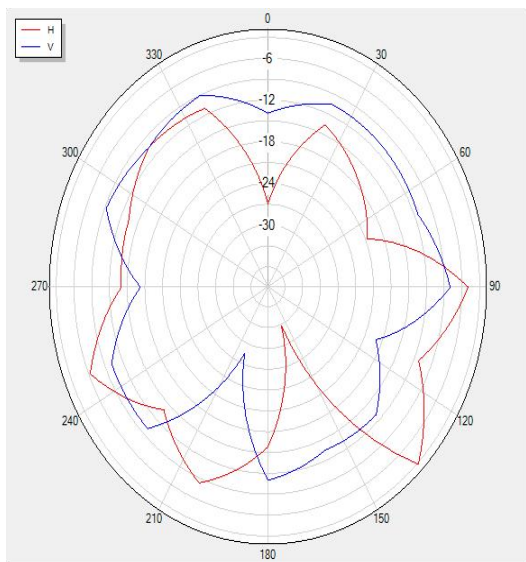
2400P90 Polar
