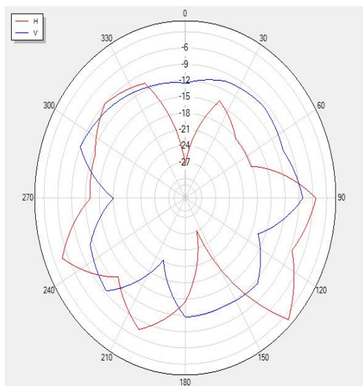
2450P90 Polar
