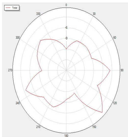
2480P90 Total
