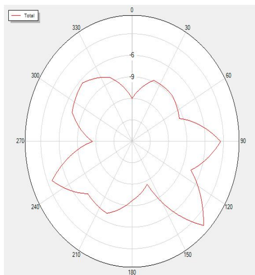
2460P90 Total
