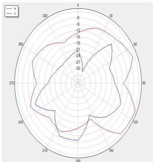
2470P0 Polar
