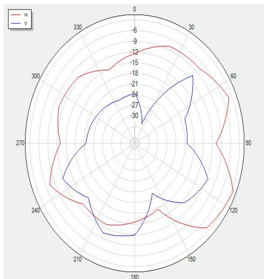
2430P0 Polar
