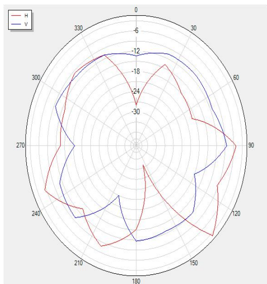
2430P90 Polar
