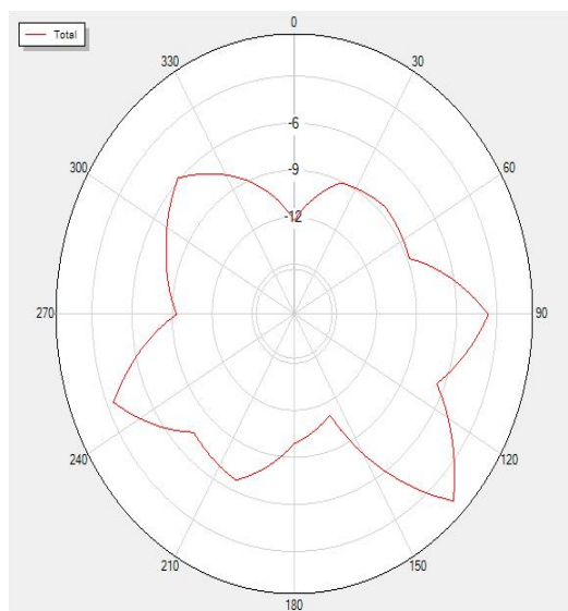
2490P90 Total
