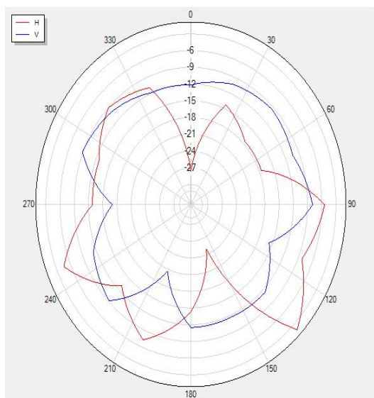
2460P90 Polar
