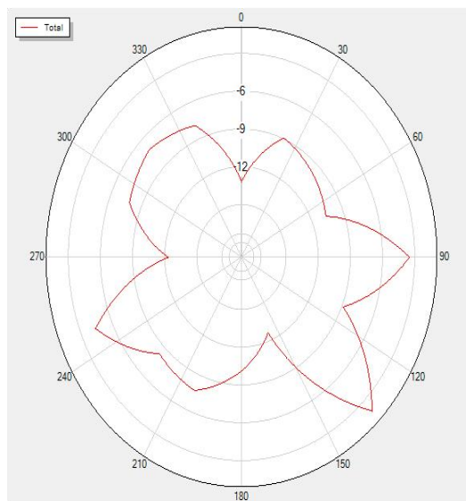
2430P90 Total
