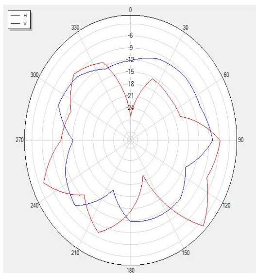
2480P90 Polar
