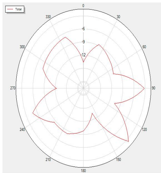
2400P90 Total
