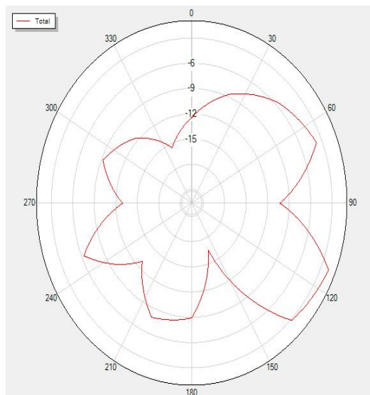
2470P0 Total
