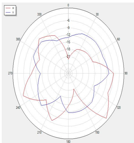
2500P90 Polar
