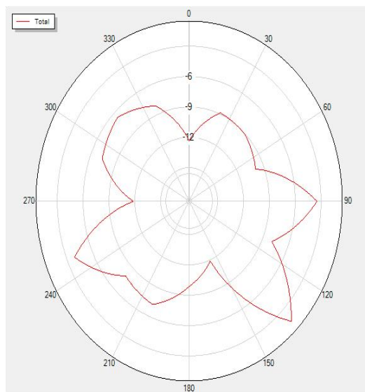
2450P90 Total
