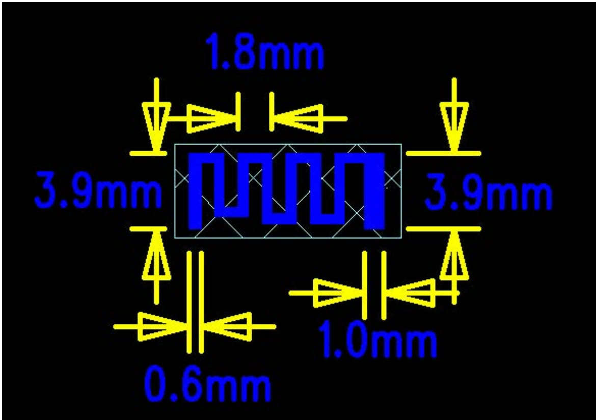
Picture of antenna
