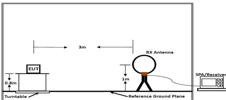
Below 30MHz
