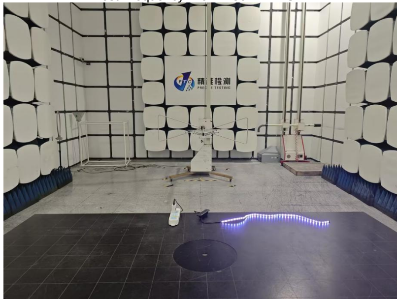
YH-255 Input: DC 5V/2A Radiated Spurious Emissions Test Frequency From 30MHz-1GHz
