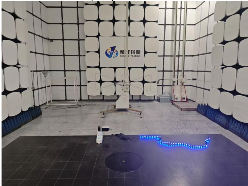
YH-256 Input: DC 12V/2A Radiated Spurious Emissions Test Frequency From 30MHz-1GHz
