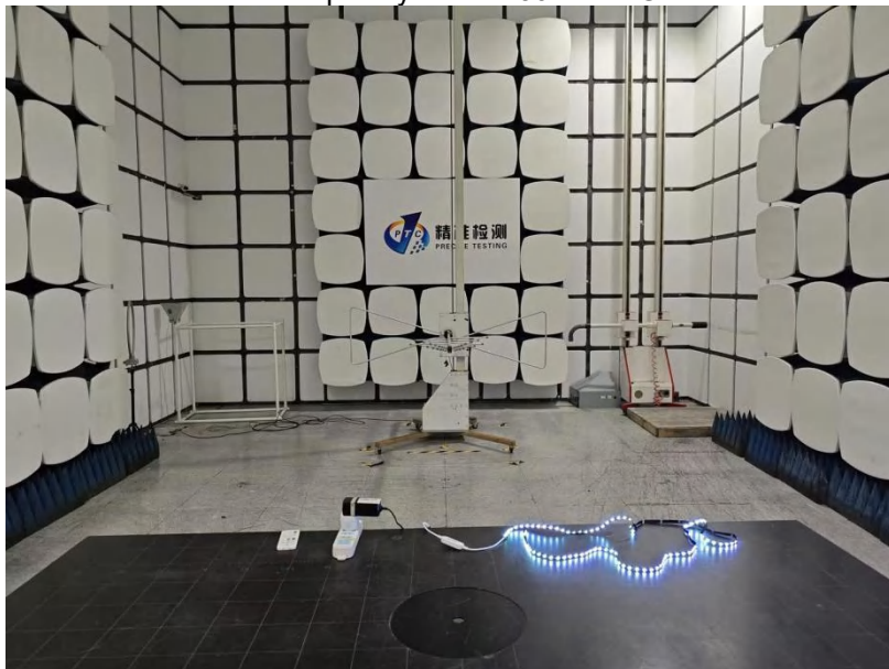
YH-6289 Input: DC 12V/2A Radiated Spurious Emissions Test Frequency From 30MHz-1GHz
