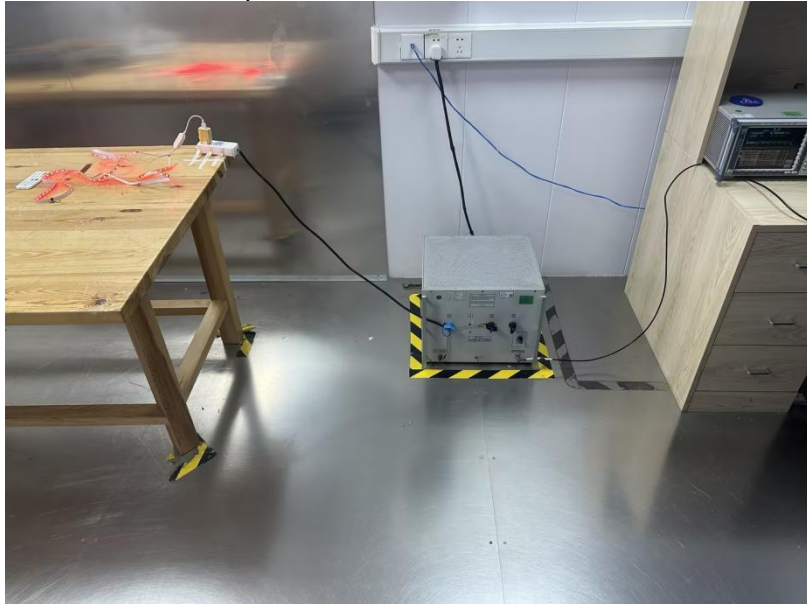
YH-6285 Input: DC 5V/2A Radiated Spurious Emissions Test Frequency From 30MHz-1GHz
