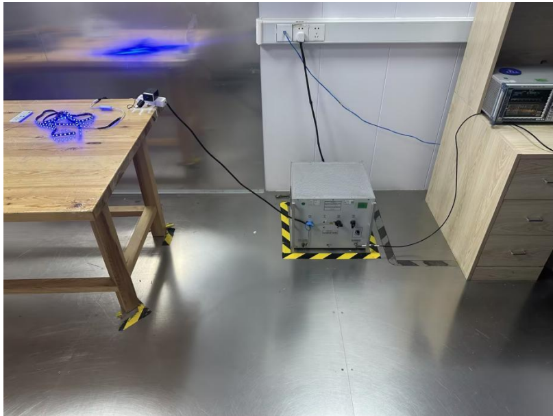
YH-6289 Input: DC 12V/2A Radiated Spurious Emissions
