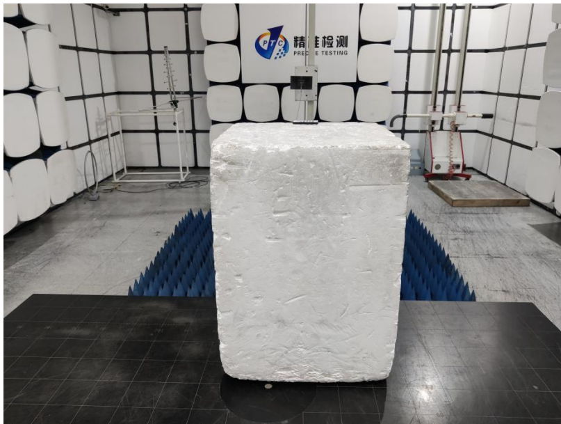
RADIATED EMISSION TEST(Above 1G)
