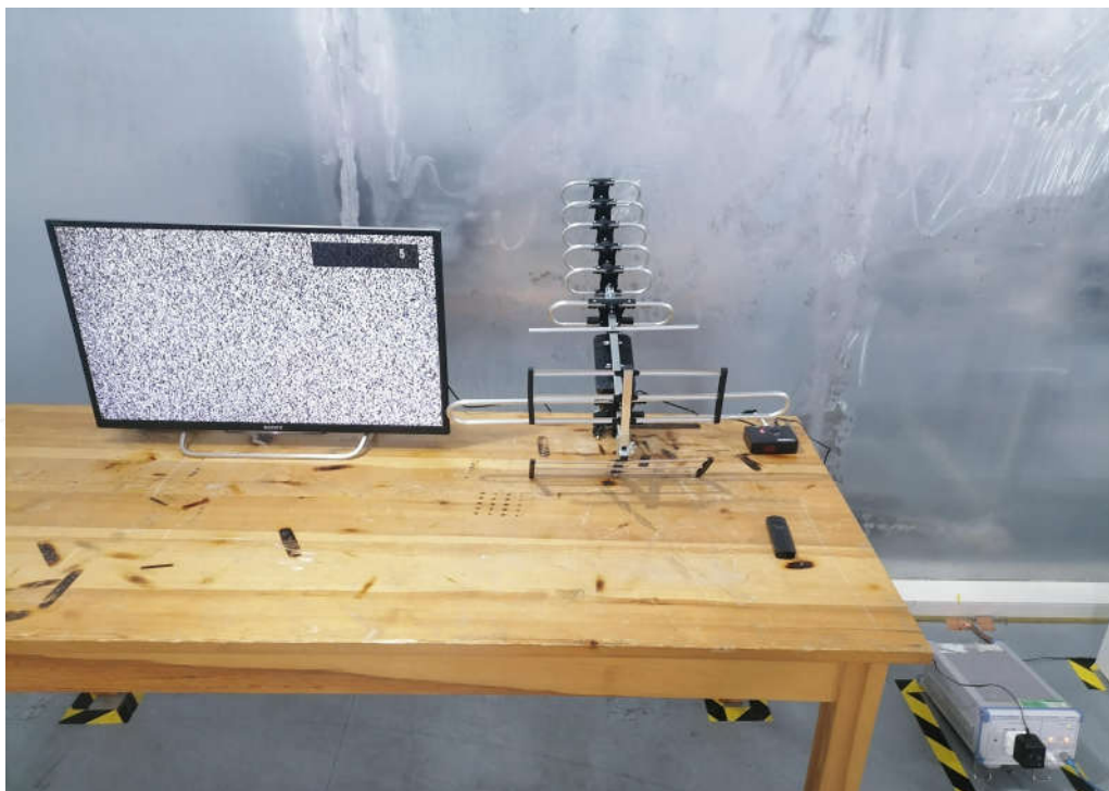
Photo of Power Line Conducted Measurement
