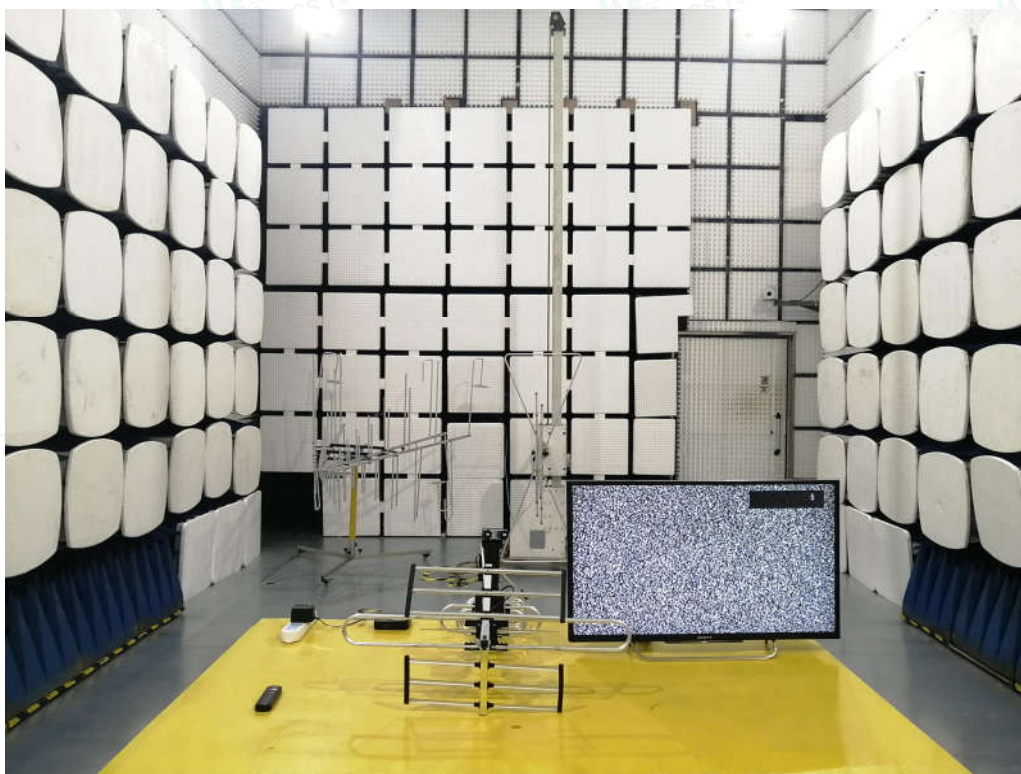
Photo of Radiated Measurement
