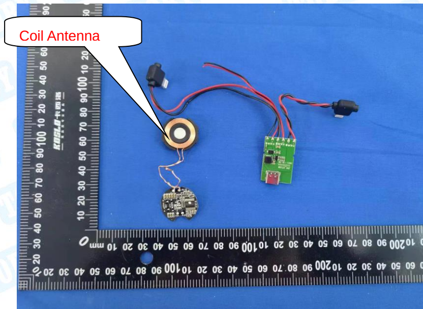
Photo 10 Appearance of PCB
