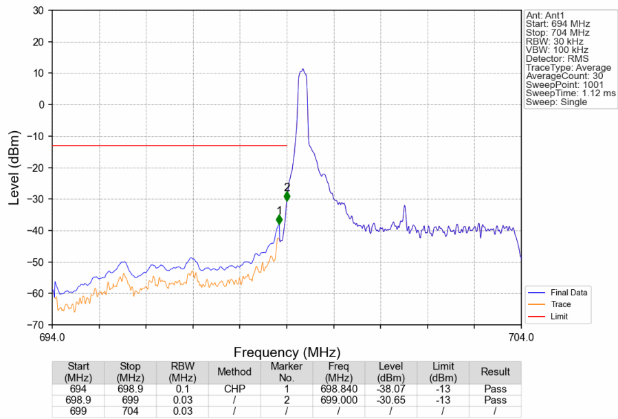
Band12_5MHz_QPSK_LCH_701.5MHz_RB_1_0_NTNV
