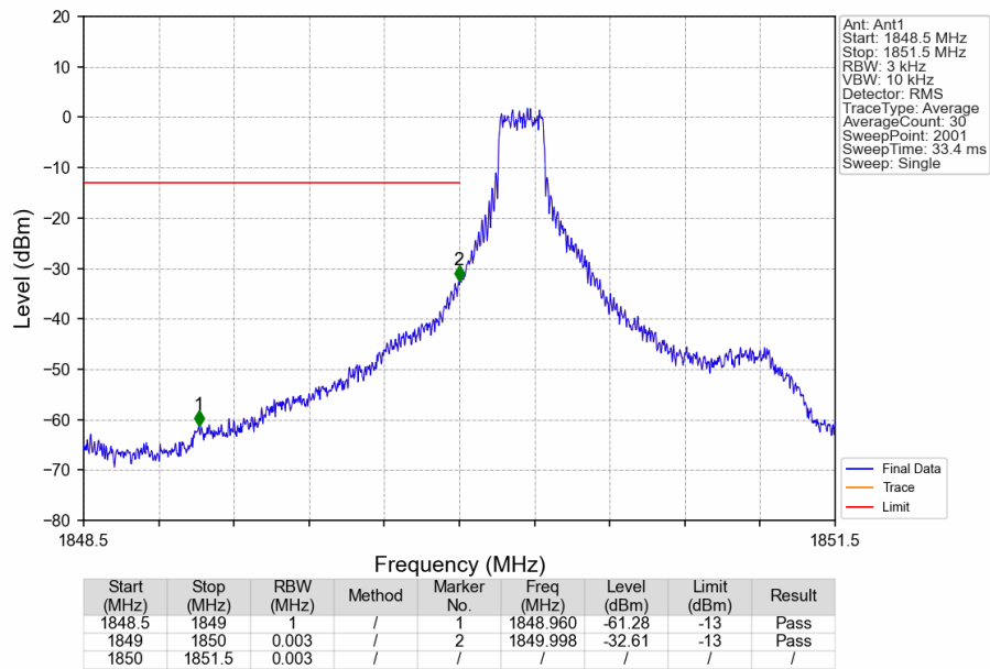
Band2_1.4MHz_QPSK_LCH_1850.7MHz_RB_1_0_NTNV
