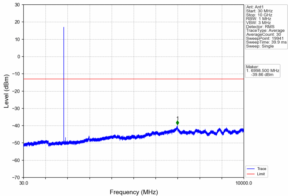
Band2_1.4MHz_QPSK_LCH_1850.7MHz_RB_1_0_NTNV
