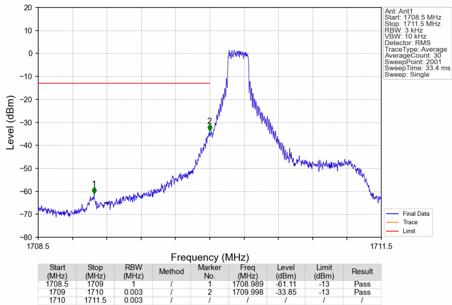
Band4_1.4MHz_QPSK_LCH_1710.7MHz_RB_1_0_NTNV
