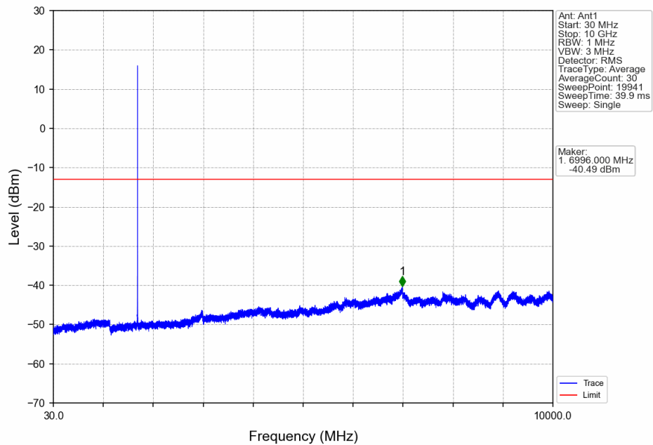
Band4_1.4MHz_QPSK_LCH_1710.7MHz_RB_1_0_NTNV
