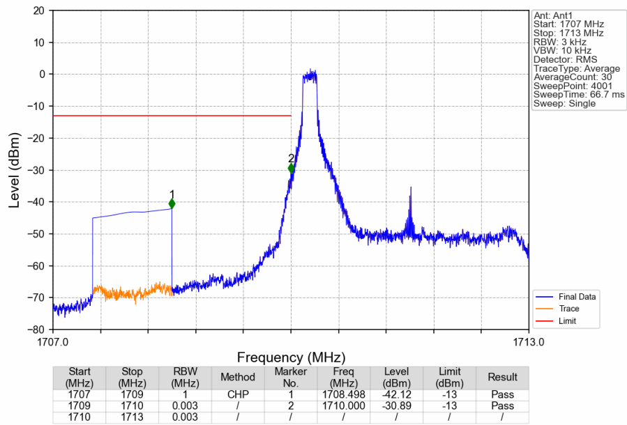
Band4_3MHz_QPSK_LCH_1711.5MHz_RB_1_0_NTNV
