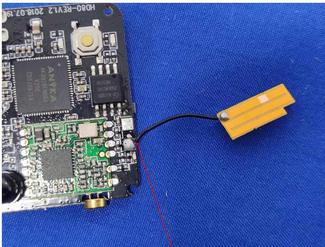
FPC antenna
