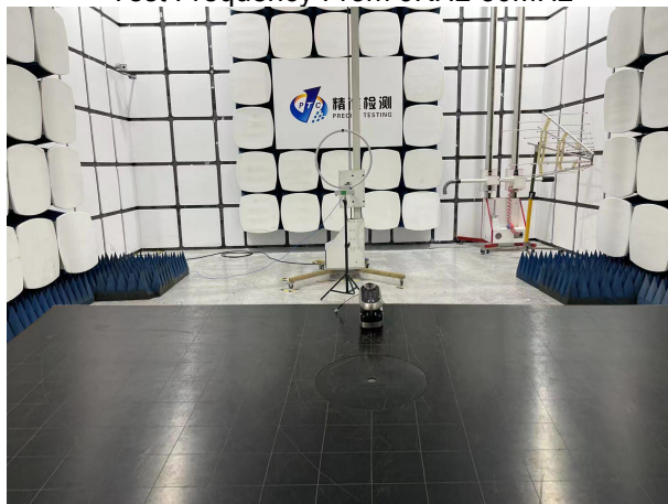
Radiated Spurious Emissions Test Frequency From 9KHz-30MHz
