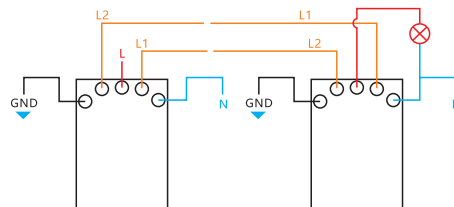
1 gang 2 way switch
