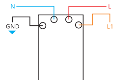
Dimmer switch
