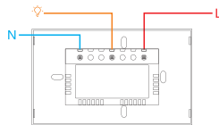
Dimmer switch
