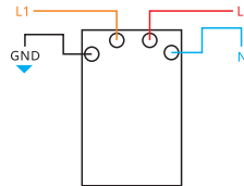
1 gang switch
