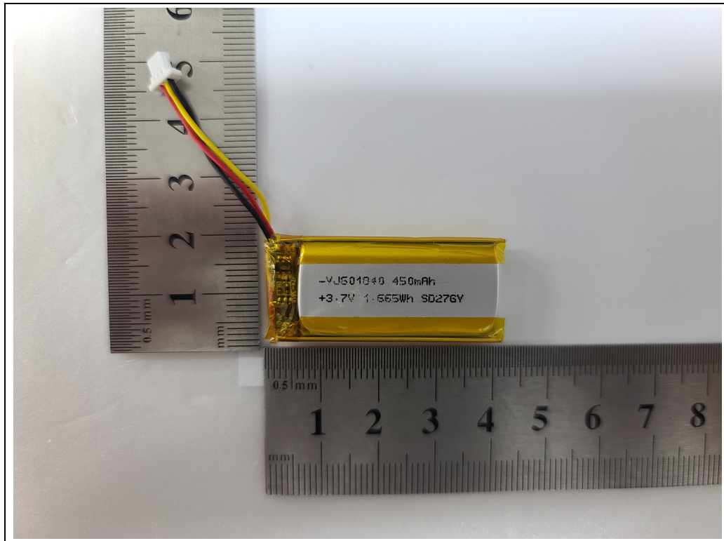
<Battery>
