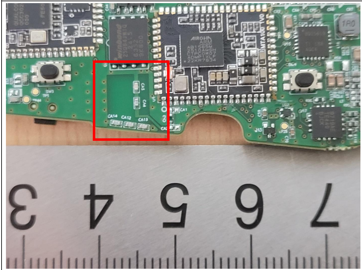
BT Antenna(BT2)
