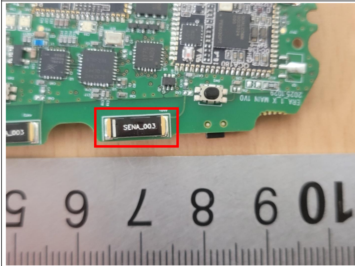
BT Antenna(BT1)
