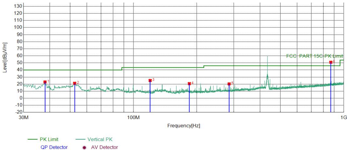
Suspected List
