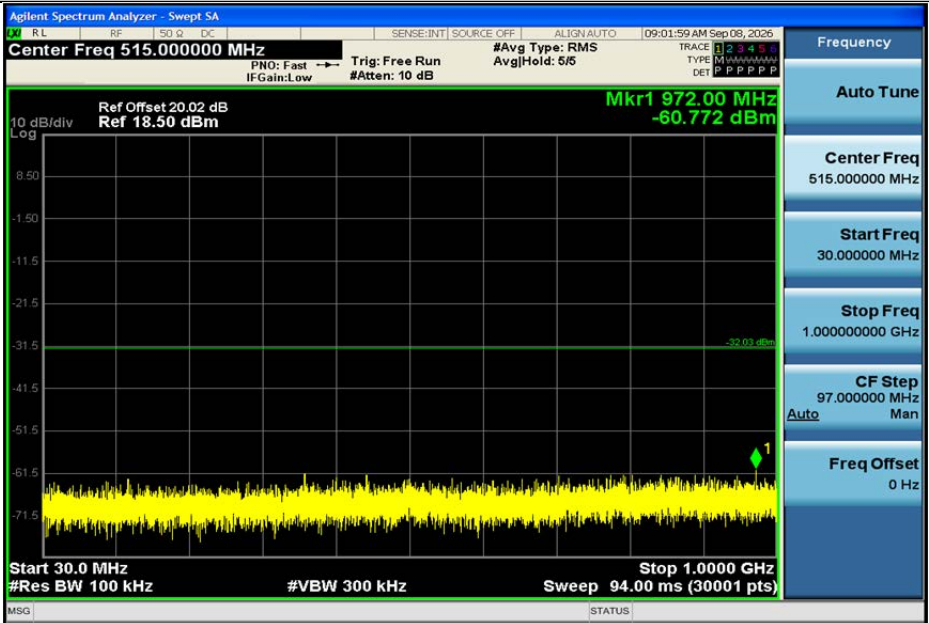
DH5-Ant1-2402-30~1000-PASS
