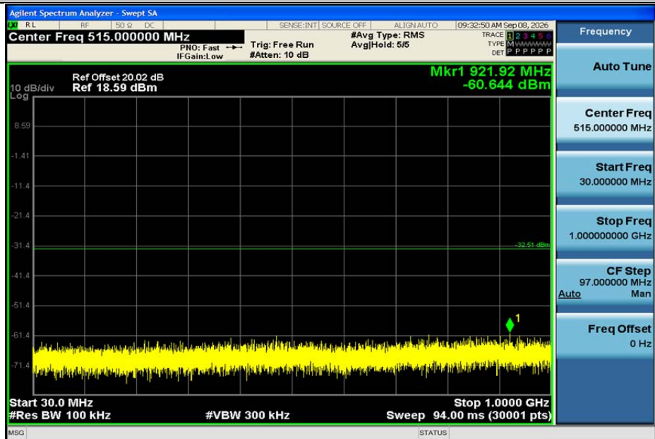
DH5-Ant1-2480-30~1000-PASS
