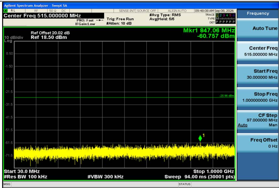
2DH5-Ant1-2402-30~1000-PASS
