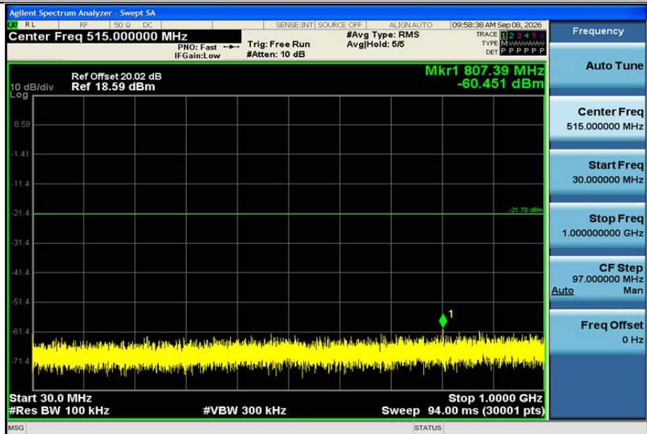
3DH5-Ant1-2480-30~1000-PASS
