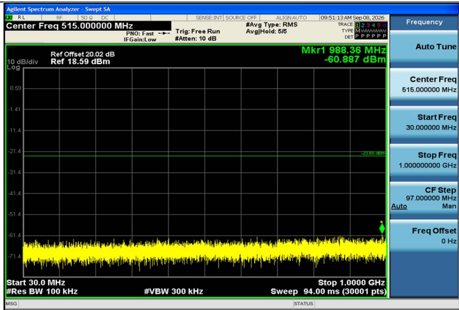
2DH5-Ant1-2480-30~1000-PASS
