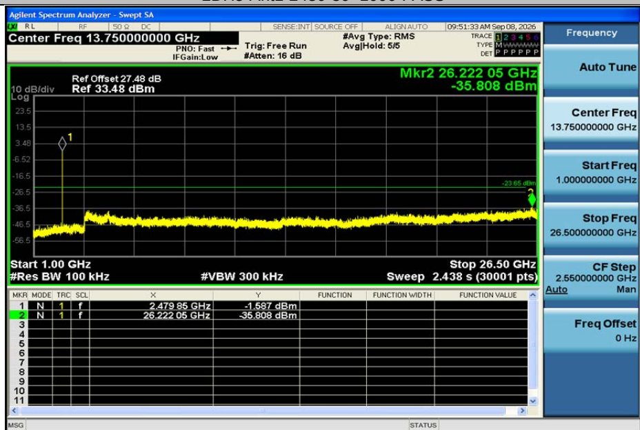
2DH5-Ant1-2480-1000~26500-PASS
