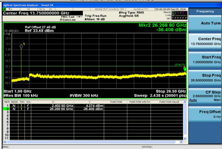
2DH5-Ant1-2402-1000~26500-PASS
