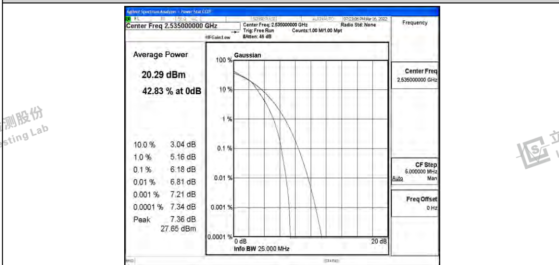
Band7-15MHz-16QAM-21375-1RB#0
