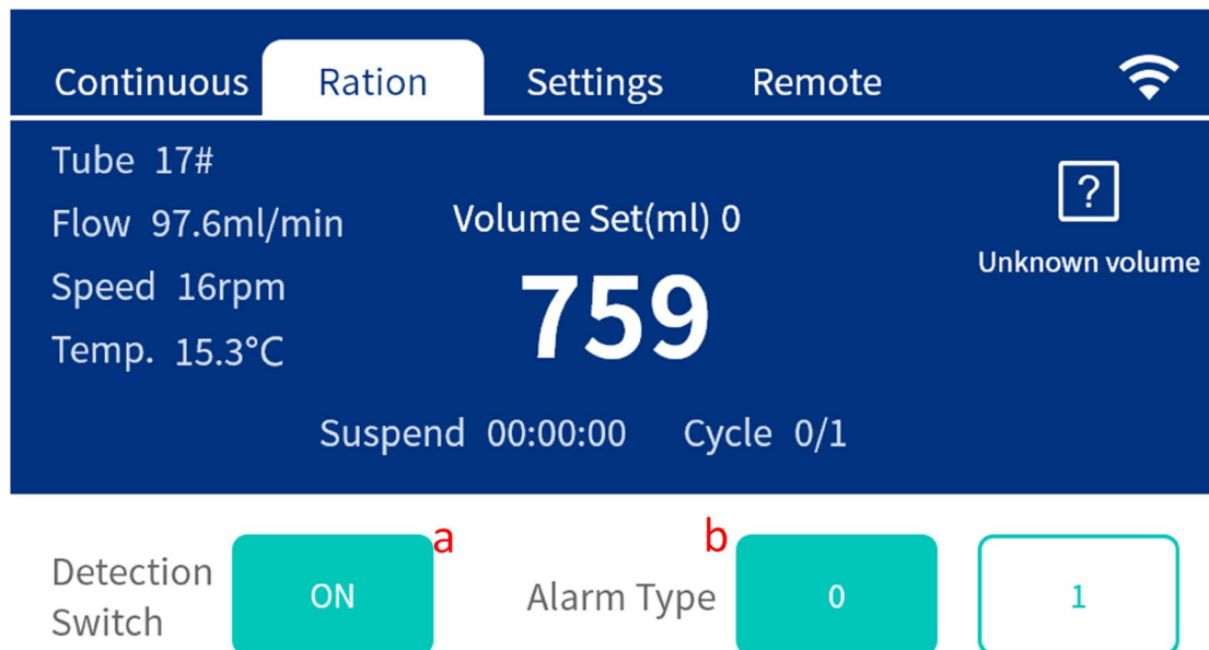
Figure 2-2-2-1 Assignment mode level detection setting
