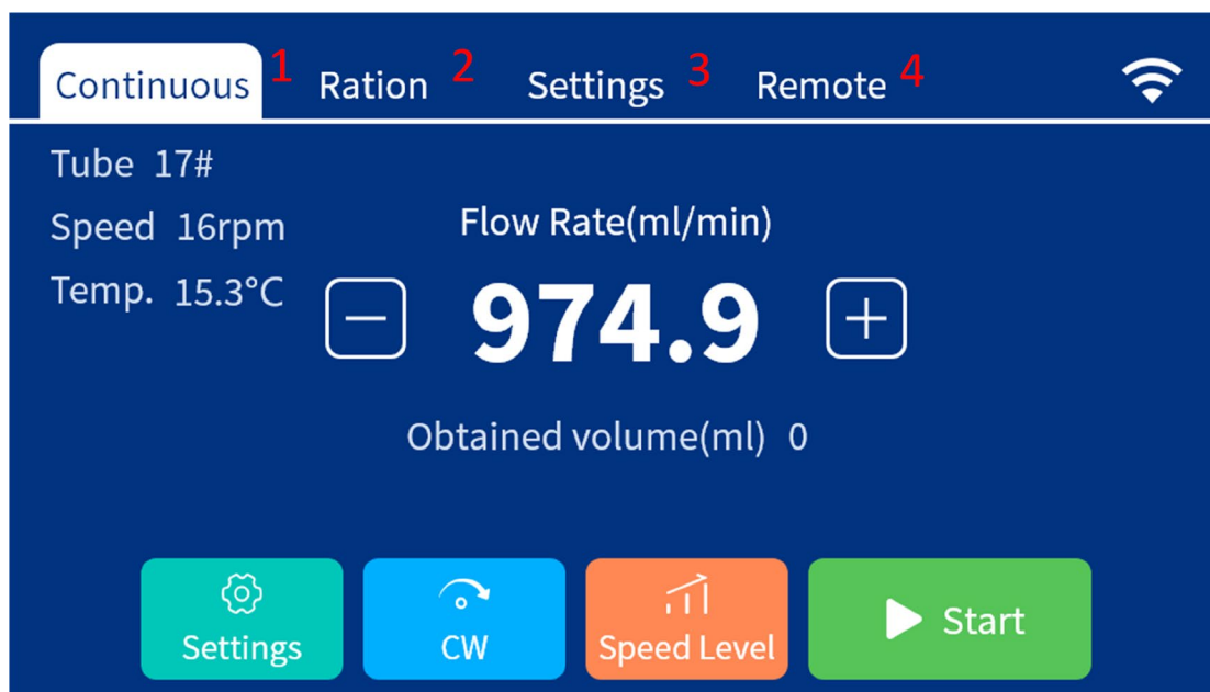
Figure 2-1 Boot interface
