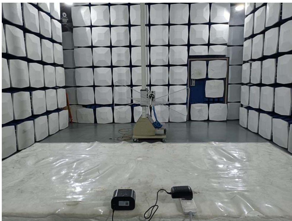
Radiated Emissions
