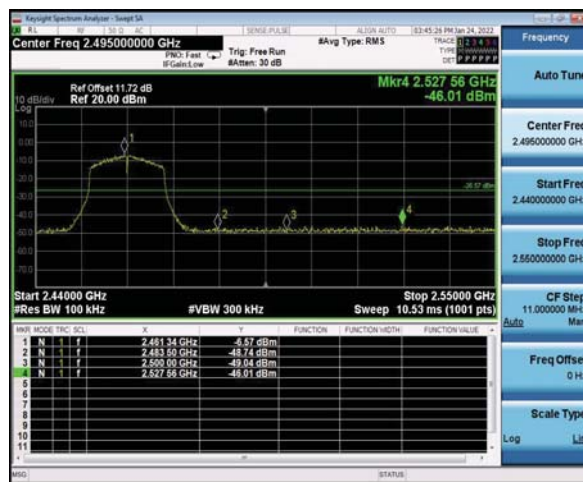
Highest channel
