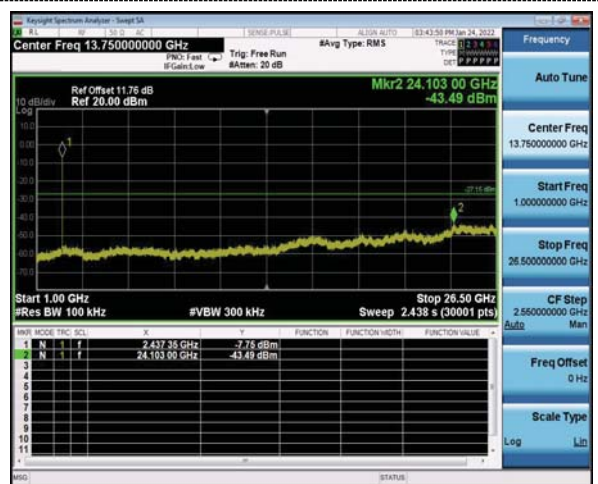
1GHz-26.5GHz
