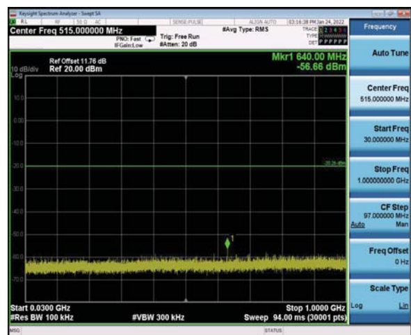
30MHz-1GHz
