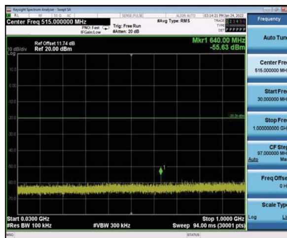
30MHz-1GHz
