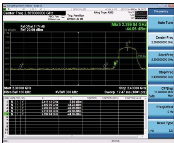
Lowest channel
