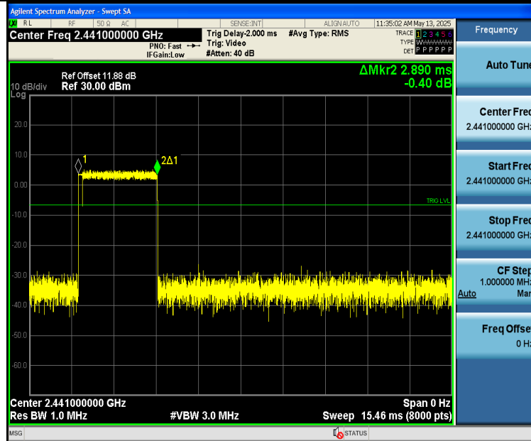
DH1-Ant2-Hop-PASS
