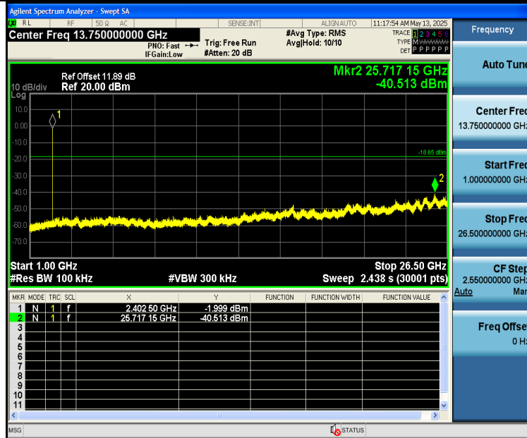
3DH5-Ant2-2441-0~Reference-PASS
