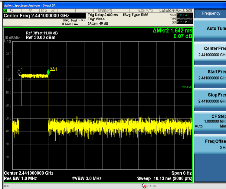
3DH3-Ant2-Hop-PASS
