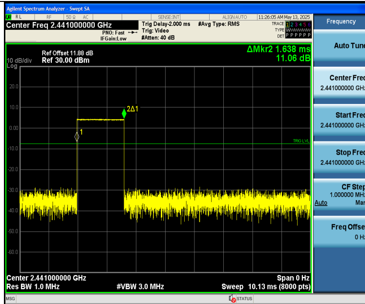
2DH3-Ant2-Hop-PASS
