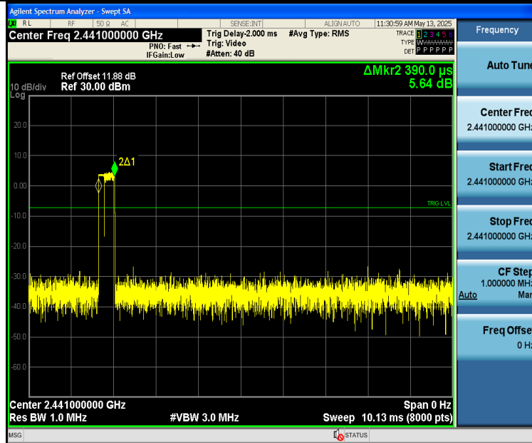
3DH1-Ant2-Hop-PASS
