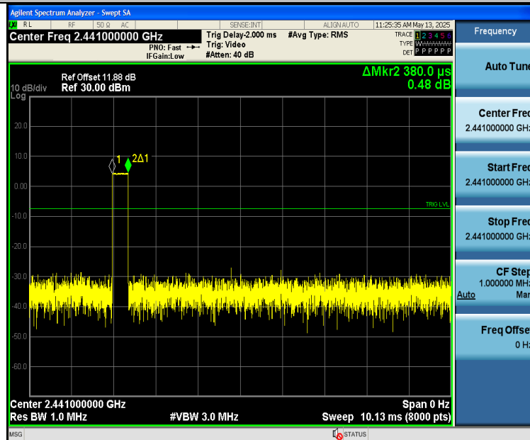
2DH1-Ant2-Hop-PASS
