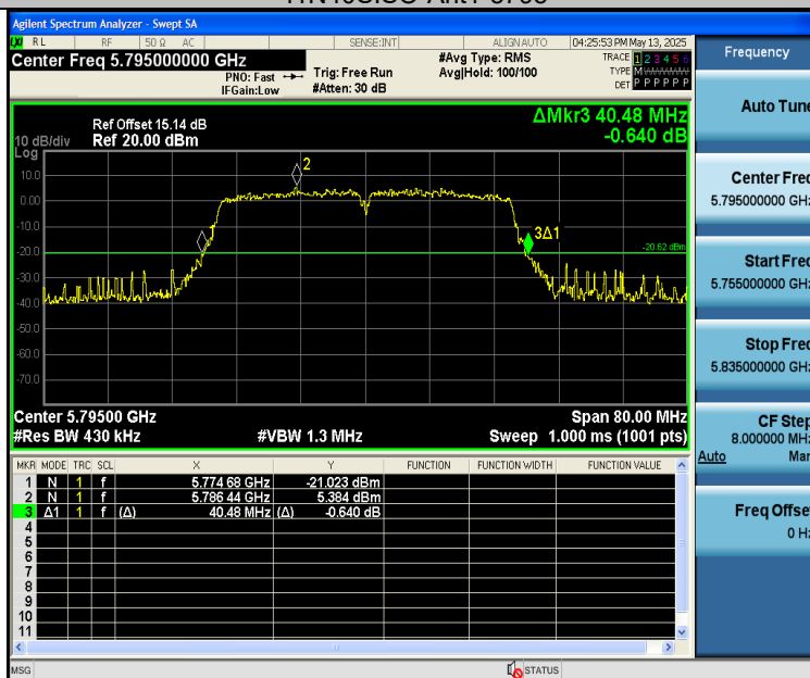
11AC20SISO-Ant1-5180
