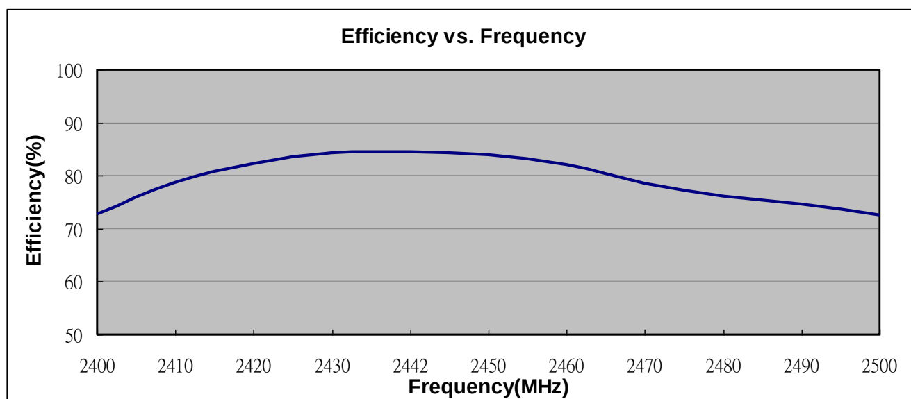
7-3. 3D Efficiency vs. Frequency
