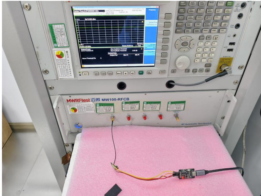
RFconducted test
