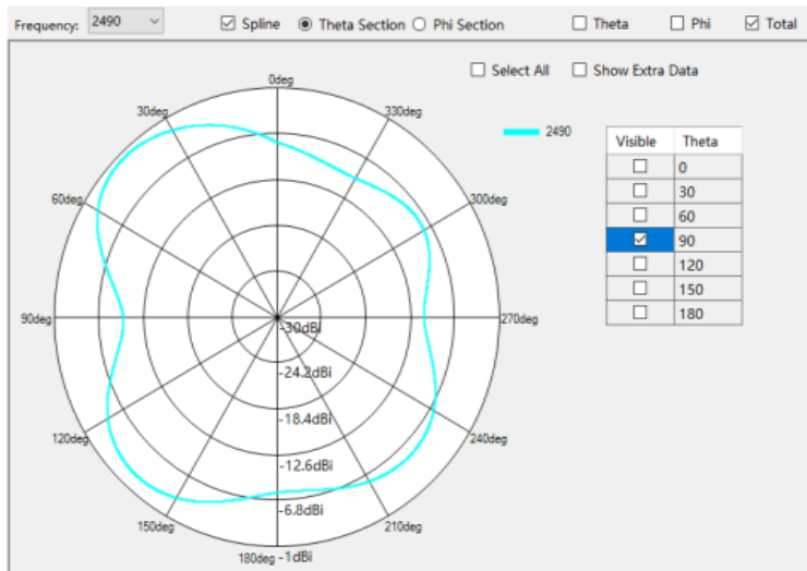
2490 MHz Gain= -0.81dBi
