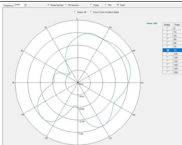
2450 MHz Gain= 3.26dBi
