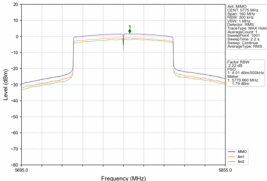
802.11ax(HEW80)_MCH_5775MHz_RU996_Left_MIMO_NTNV
