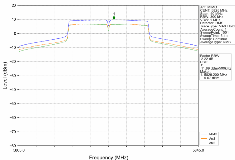
802.11ac(VHT20)_HCH_5825MHz_MIMO_NTNV
