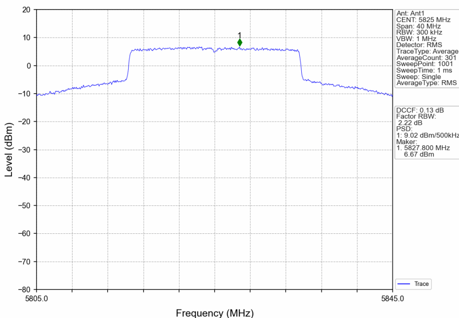
802.11ax(HEW20)_HCH_5825MHz_RU242_Left_Ant1_NTNV
