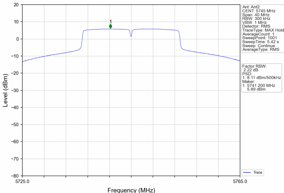
802.11ac(VHT20)_LCH_5745MHz_MIMO_NTNV
