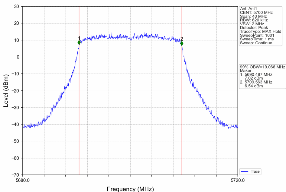
802.11ax(HEW20)_HCH_5700MHz_RU242_Left_Ant1_NTNV
