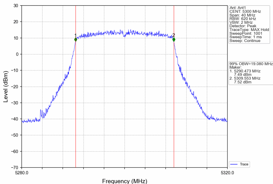
802.11ax(HEW20)_MCH_5300MHz_RU242_Left_Ant1_NTNV
