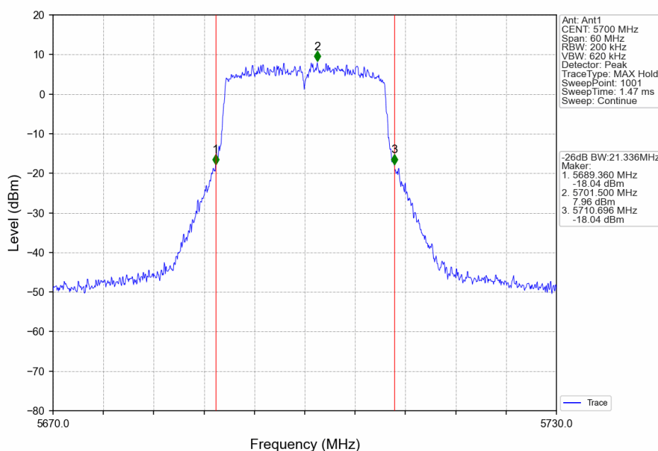
802.11ax(HEW20)_HCH_5700MHz_RU242_Left_Ant1_NTNV
