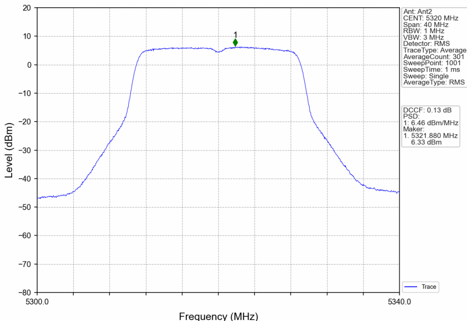
802.11ac(VHT20)_HCH_5320MHz_MIMO_NTNV
