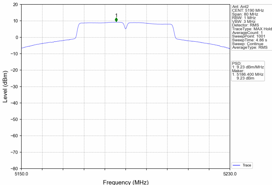
802.11n(HT40)_LCH_5190MHz_MIMO_NTNV
